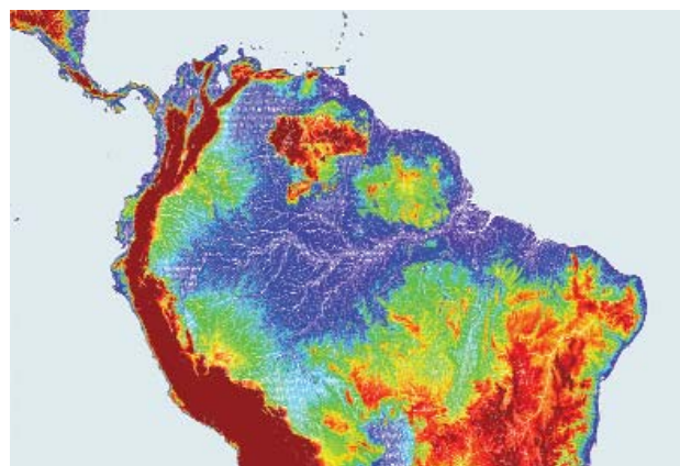
Figure 7. The Amazon River Basin as observed by ERS-1 radar altimeter (European Space Agency, www.esa.int/esaEO/SEMDHU2VQUD_planet1.html ).
